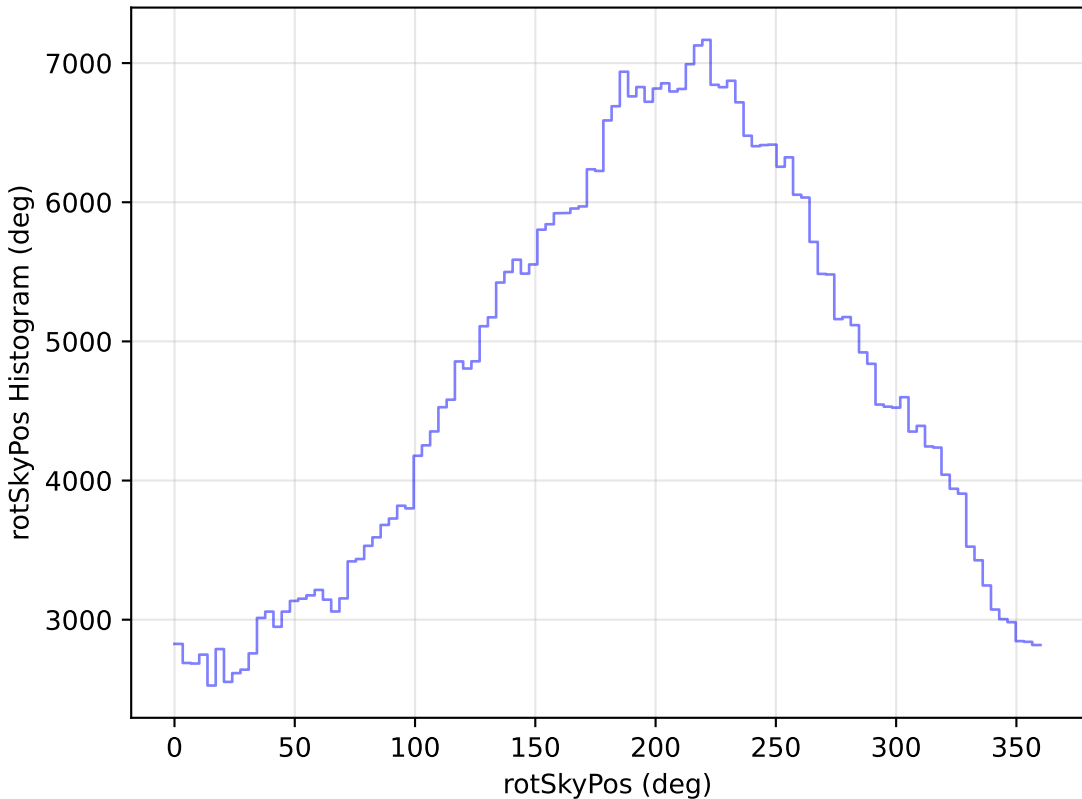
ddf_loaded_fl1_v3.4_10yrs WFD r band: rotSkyPos Histogram
