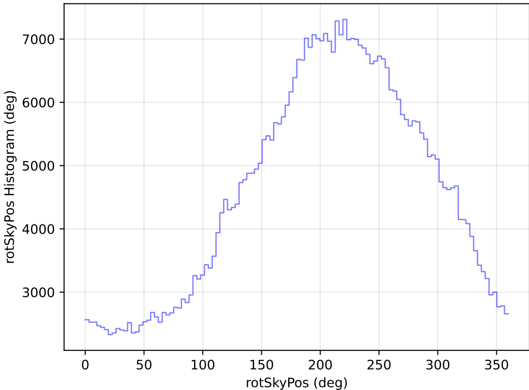
ddf_loaded_fl1_v3.4_10yrs WFD i band: rotSkyPos Histogram
