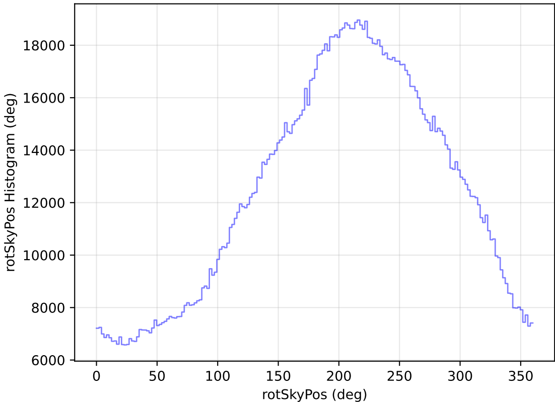
ddf_loaded_fl1_v3.4_10yrs WFD all bands: rotSkyPos Histogram
