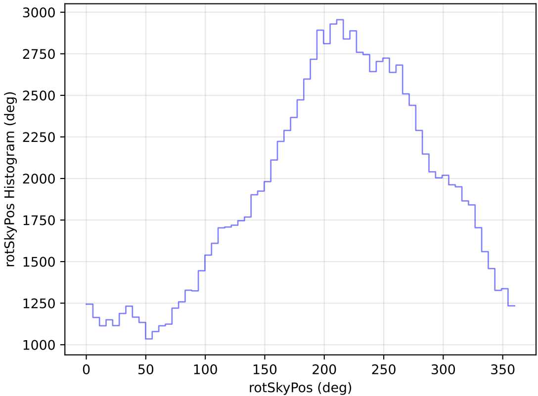
ddf_loaded_fl1_v3.4_10yrs All sky u band: rotSkyPos Histogram
