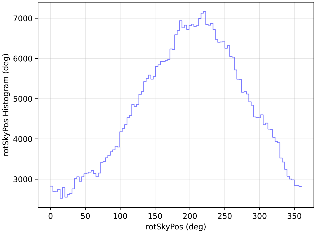
ddf_loaded_fl1_v3.4_10yrs All sky r band: rotSkyPos Histogram
