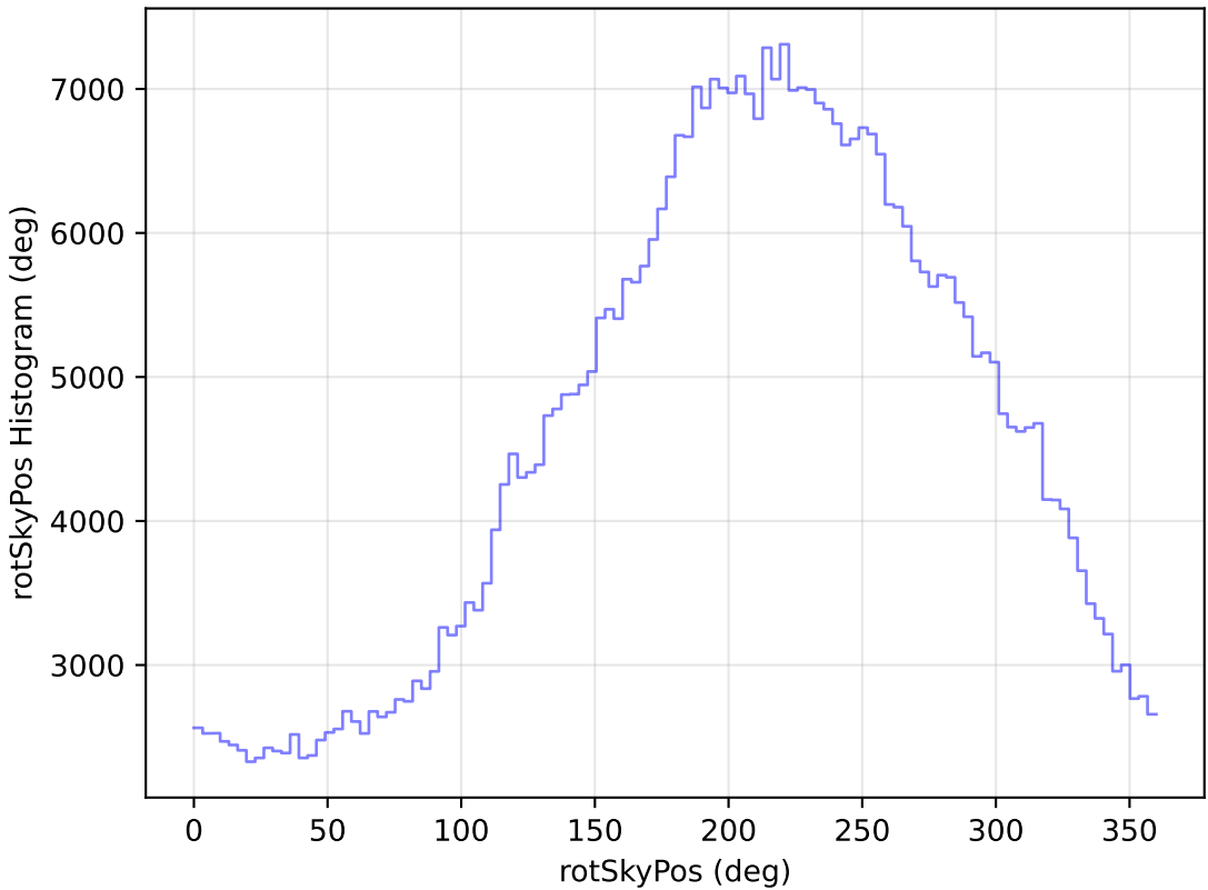
ddf_loaded_fl1_v3.4_10yrs All sky i band: rotSkyPos Histogram
