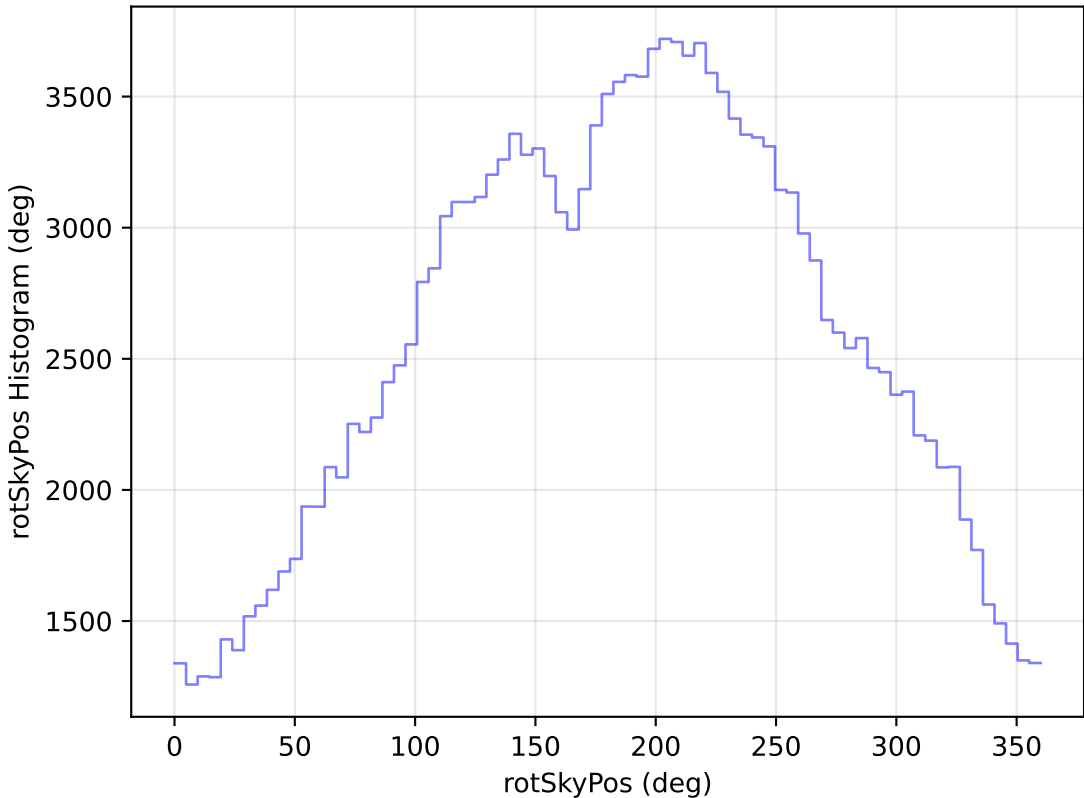
ddf_loaded_fl1_v3.4_10yrs All sky g band: rotSkyPos Histogram
