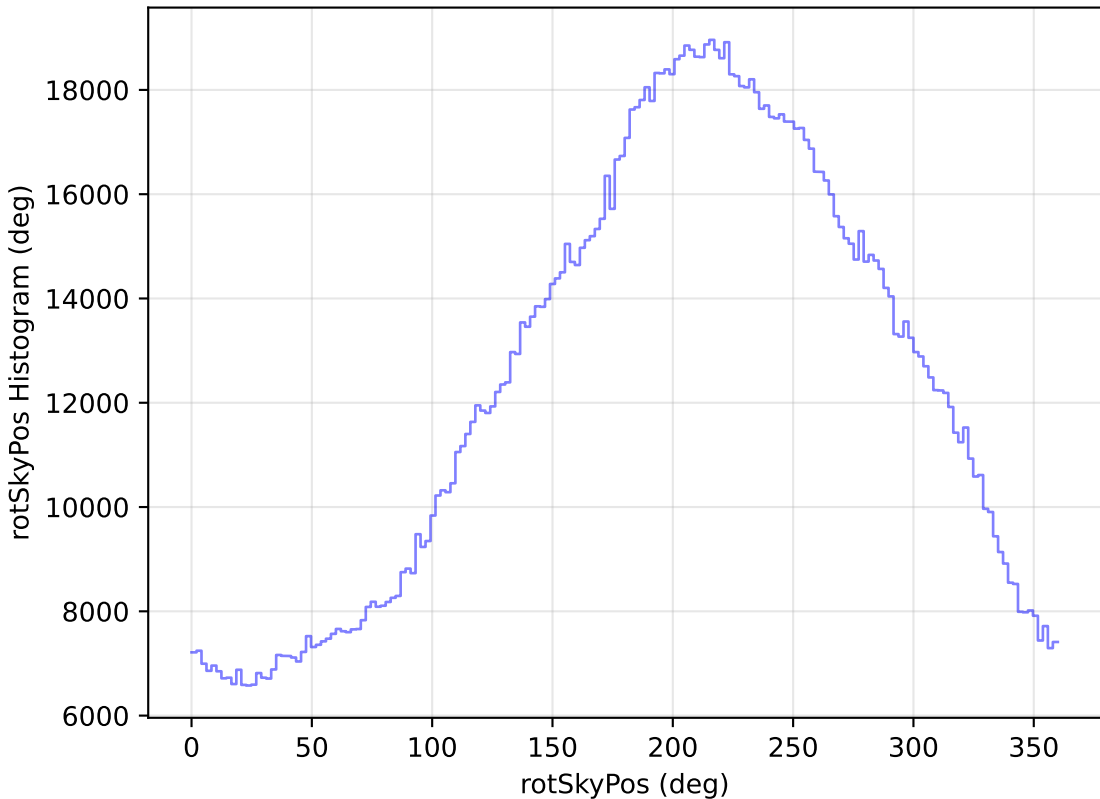
ddf_loaded_fl1_v3.4_10yrs All sky all bands: rotSkyPos Histogram
