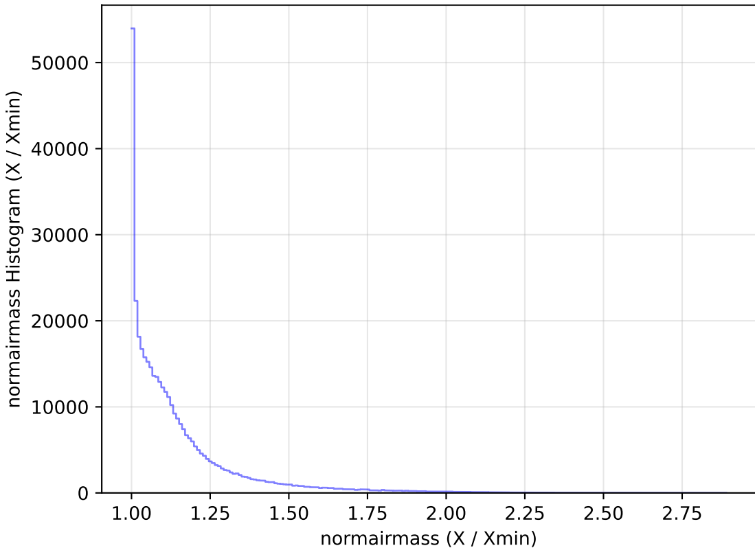
ddf_loaded_fl1_v3.4_10yrs WFD y band: normairmass Histogram
