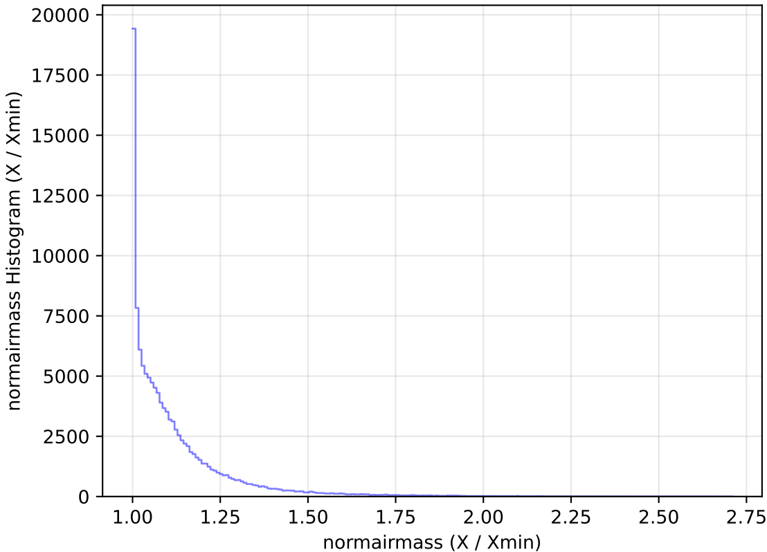
ddf_loaded_fl1_v3.4_10yrs WFD u band: normairmass Histogram
