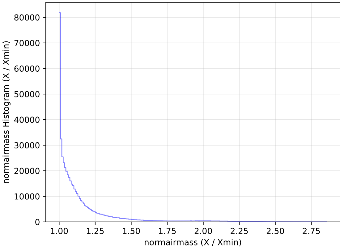
ddf_loaded_fl1_v3.4_10yrs WFD r band: normairmass Histogram
