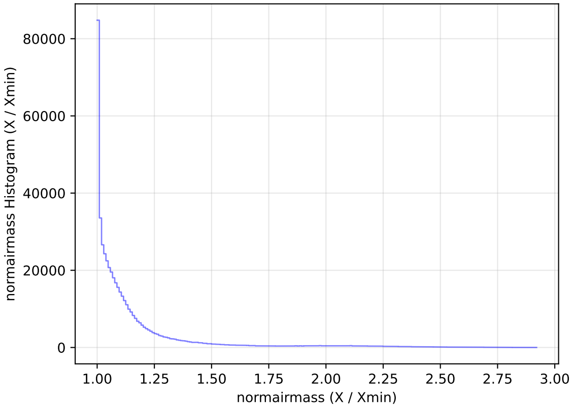
ddf_loaded_fl1_v3.4_10yrs WFD i band: normairmass Histogram
