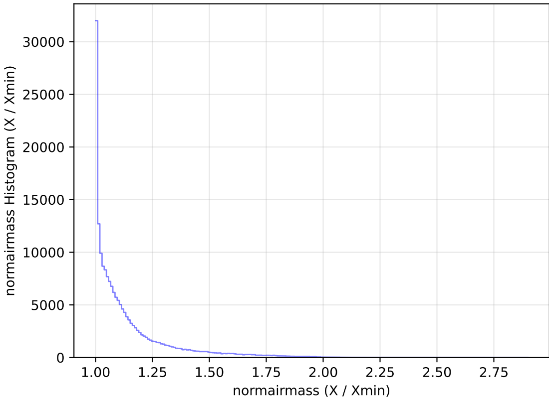
ddf_loaded_fl1_v3.4_10yrs WFD g band: normairmass Histogram
