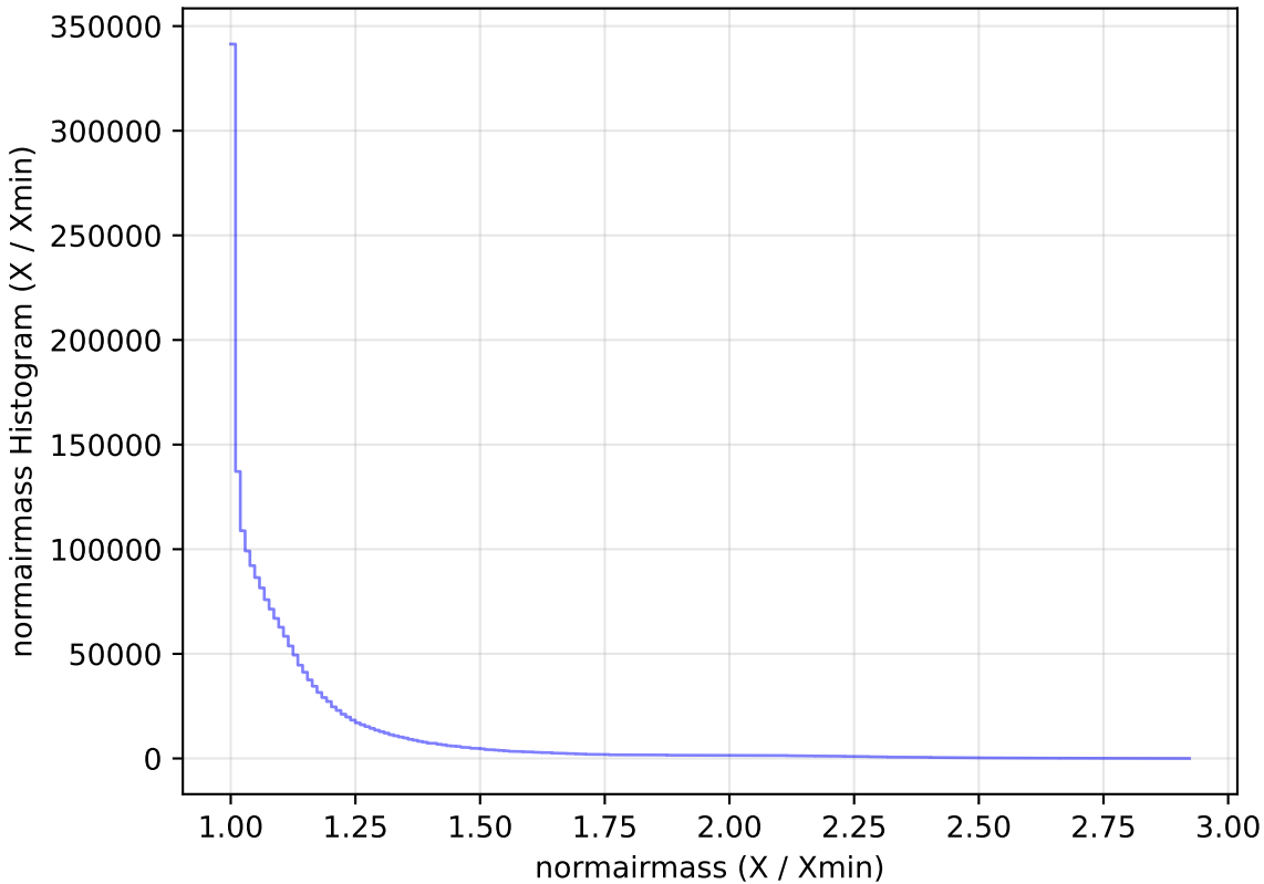
ddf_loaded_fl1_v3.4_10yrs WFD all bands: normairmass Histogram
