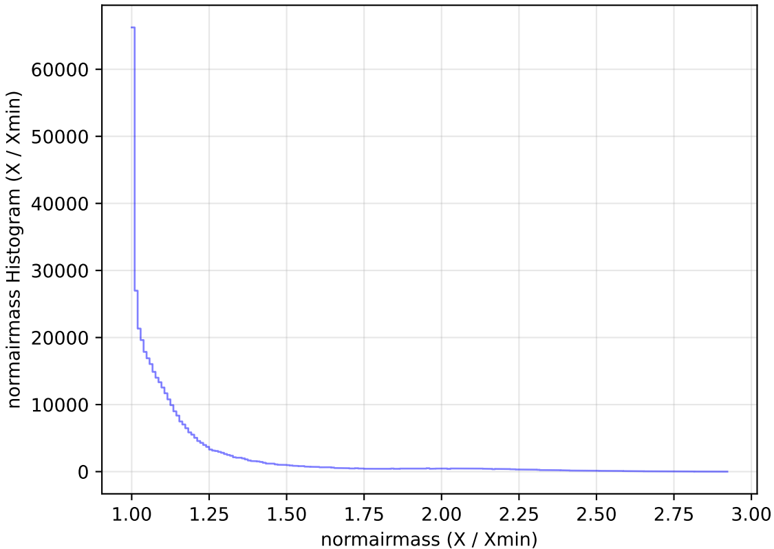
ddf_loaded_fl1_v3.4_10yrs All sky z band: normairmass Histogram
