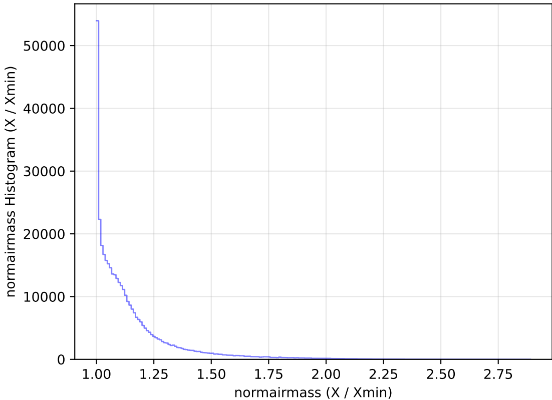
ddf_loaded_fl1_v3.4_10yrs All sky y band: normairmass Histogram
