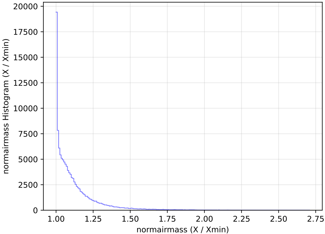
ddf_loaded_fl1_v3.4_10yrs All sky u band: normairmass Histogram
