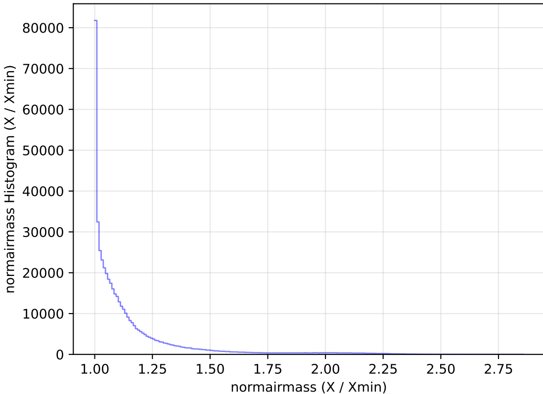
ddf_loaded_fl1_v3.4_10yrs All sky r band: normairmass Histogram
