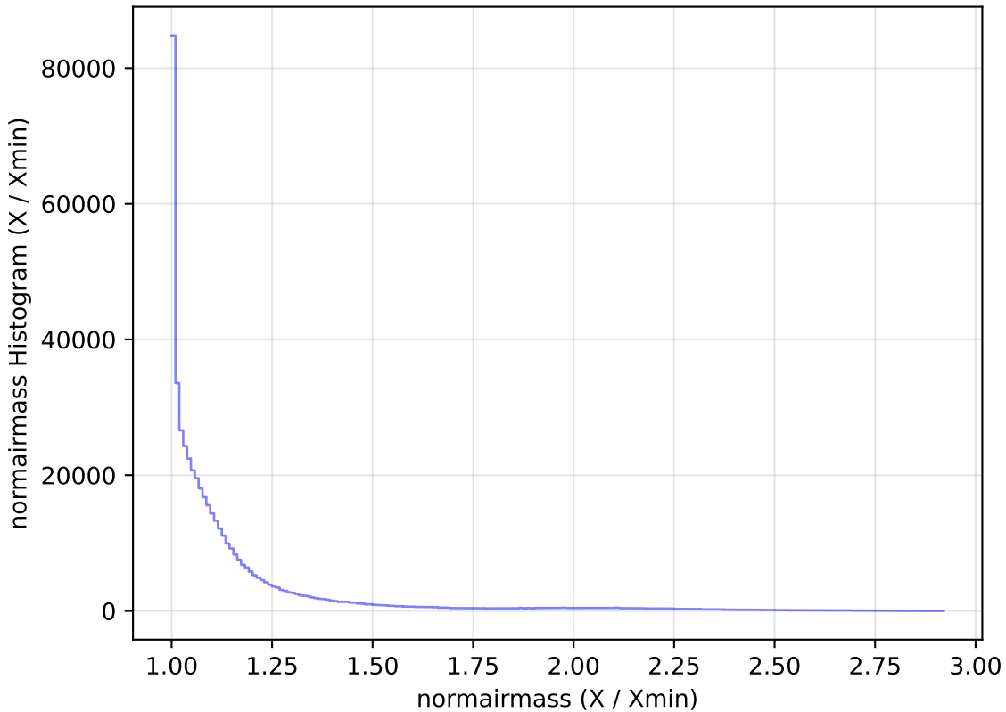
ddf_loaded_fl1_v3.4_10yrs All sky i band: normairmass Histogram
