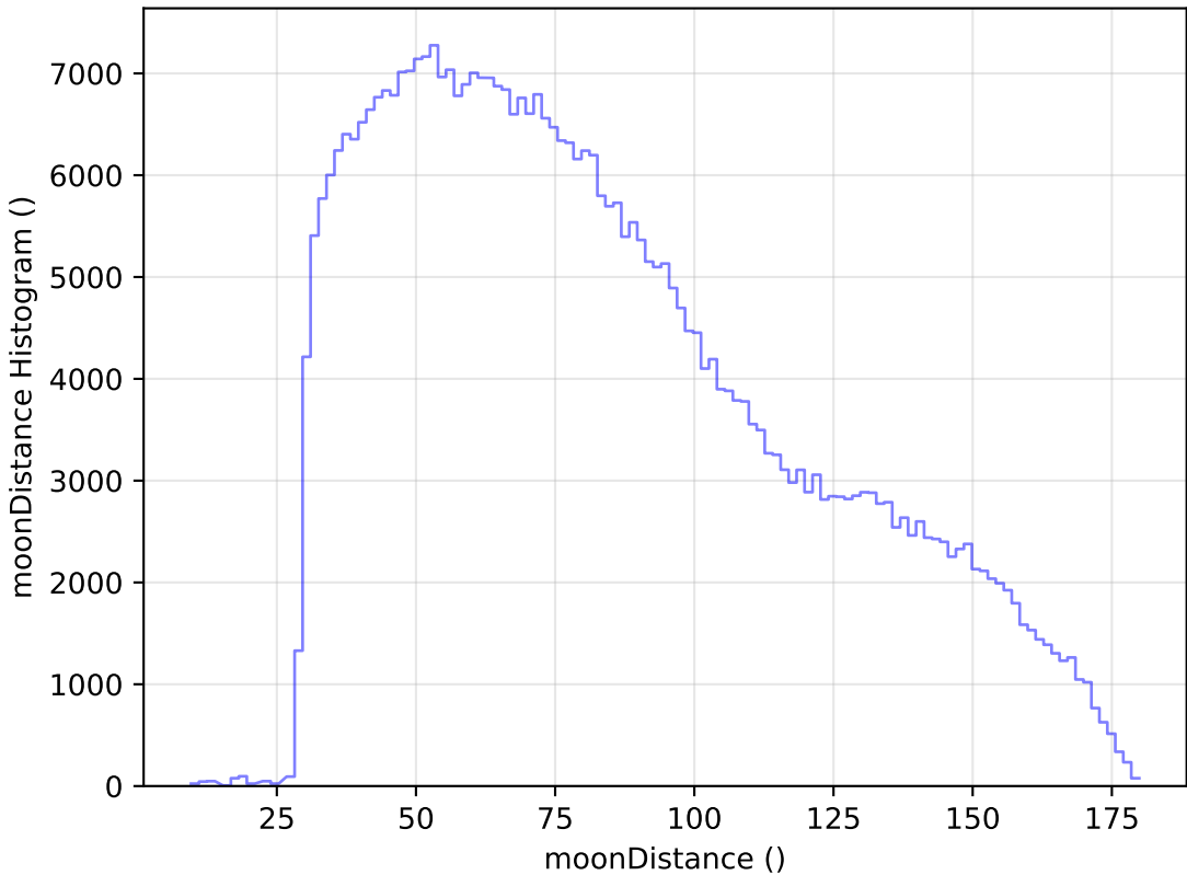
ddf_loaded_fl1_v3.4_10yrs WFD z band: moonDistance Histogram
