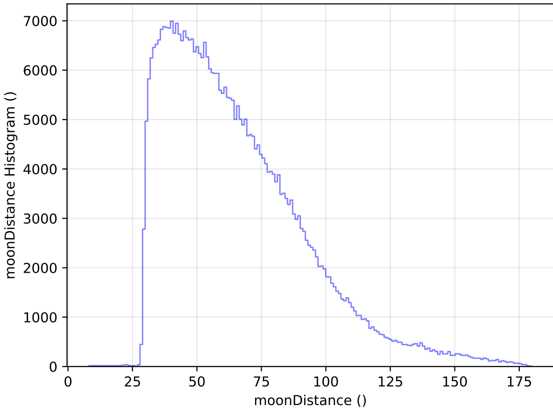
ddf_loaded_fl1_v3.4_10yrs WFD y band: moonDistance Histogram
