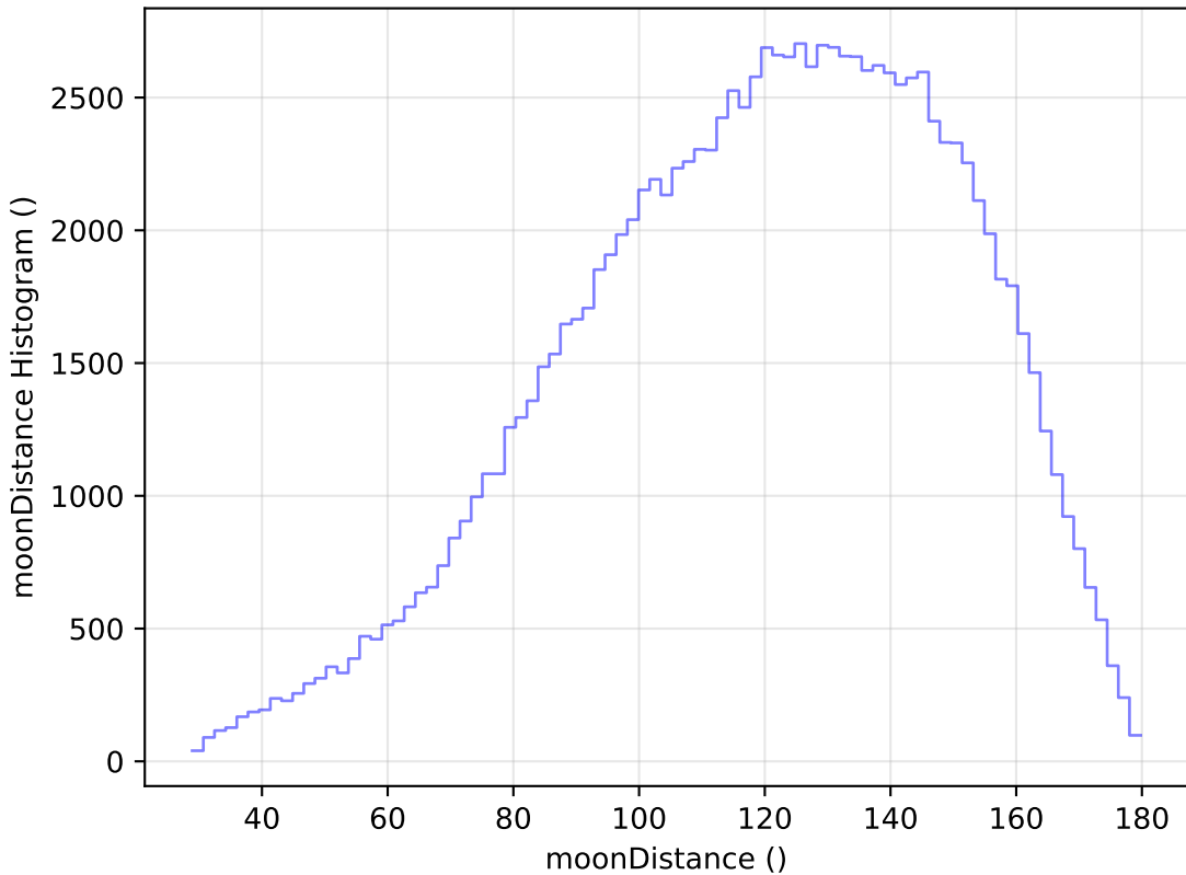
ddf_loaded_fl1_v3.4_10yrs WFD u band: moonDistance Histogram
