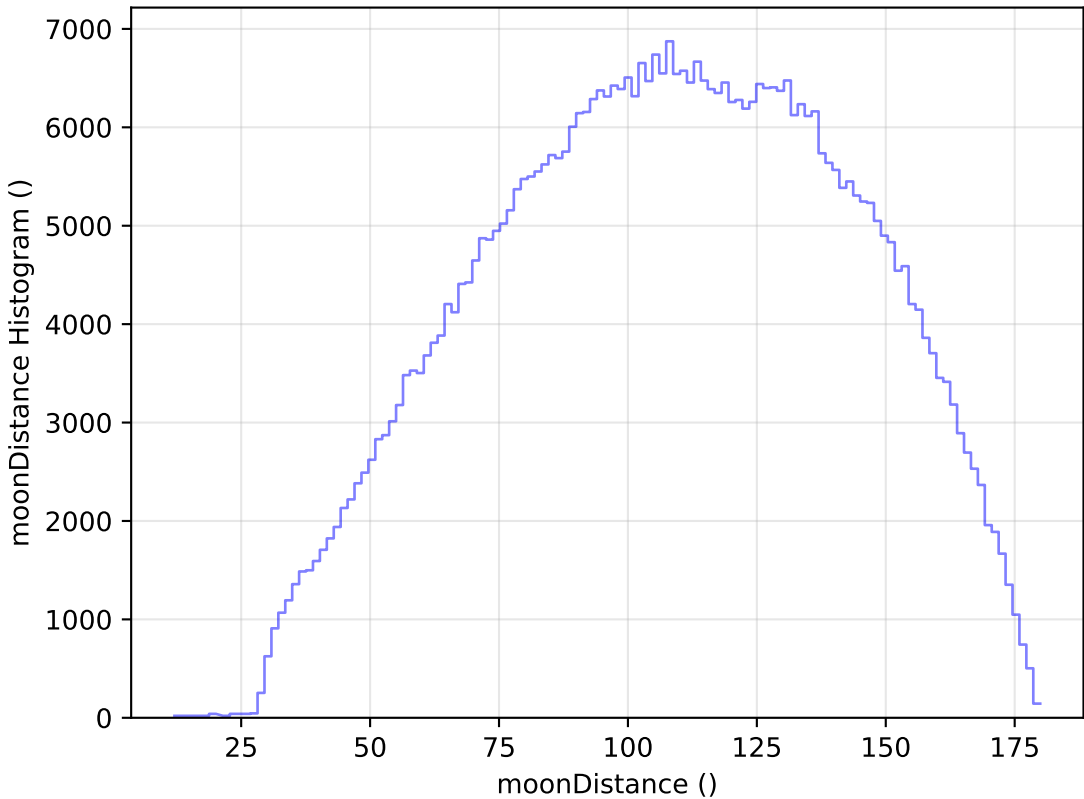
ddf_loaded_fl1_v3.4_10yrs WFD r band: moonDistance Histogram
