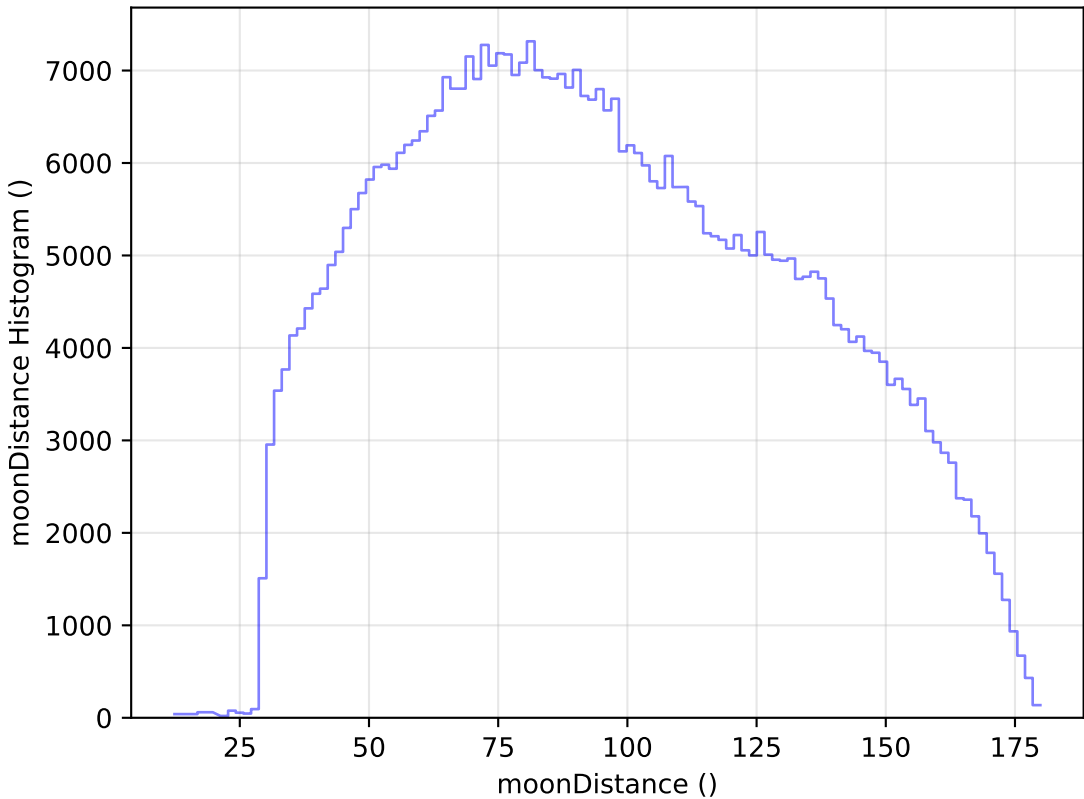
ddf_loaded_fl1_v3.4_10yrs WFD i band: moonDistance Histogram
