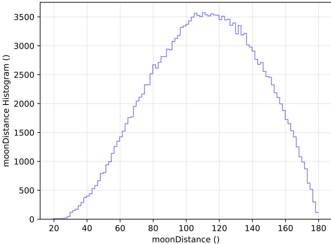
ddf_loaded_fl1_v3.4_10yrs WFD g band: moonDistance Histogram
