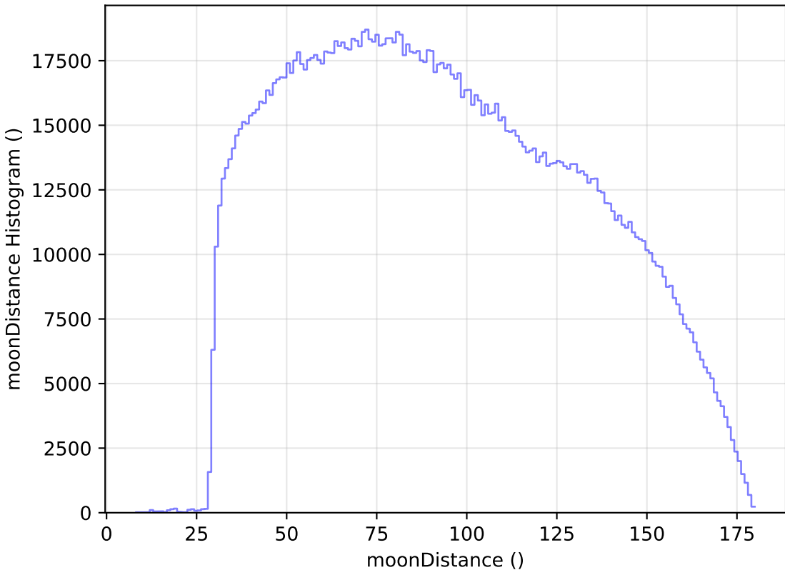
ddf_loaded_fl1_v3.4_10yrs WFD all bands: moonDistance Histogram
