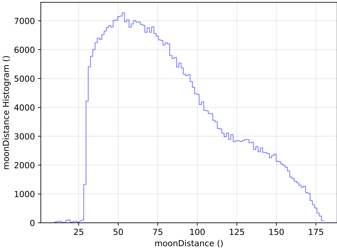
ddf_loaded_fl1_v3.4_10yrs All sky z band: moonDistance Histogram
