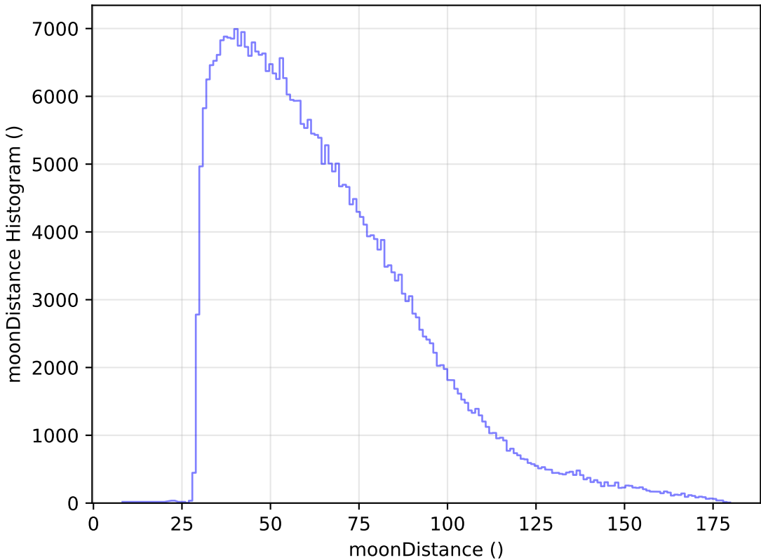
ddf_loaded_fl1_v3.4_10yrs All sky y band: moonDistance Histogram
