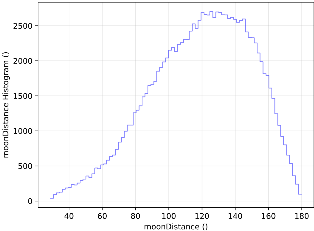
ddf_loaded_fl1_v3.4_10yrs All sky u band: moonDistance Histogram
