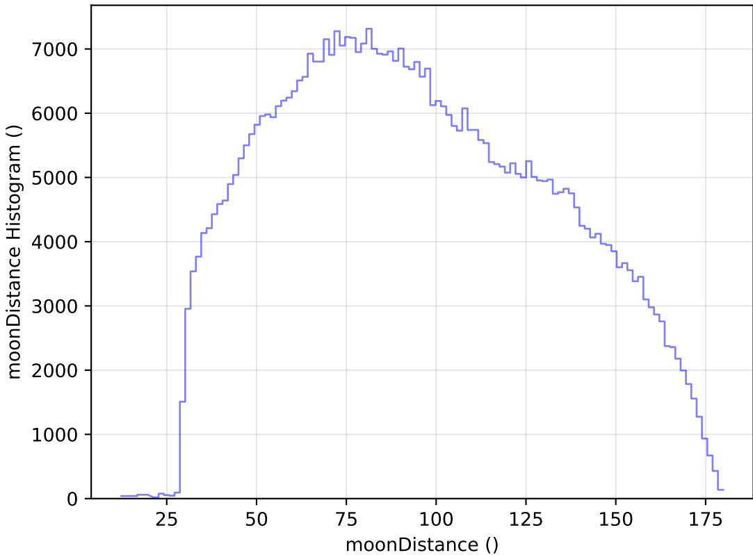
ddf_loaded_fl1_v3.4_10yrs All sky i band: moonDistance Histogram
