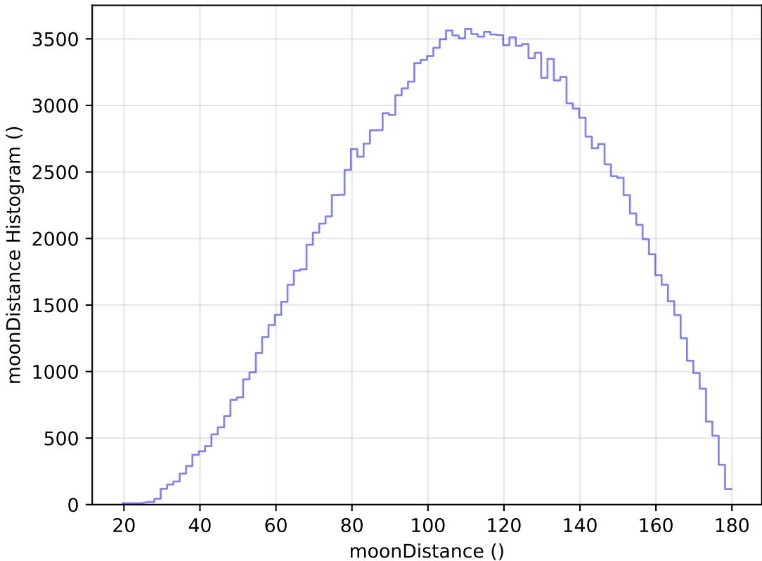
ddf_loaded_fl1_v3.4_10yrs All sky g band: moonDistance Histogram
