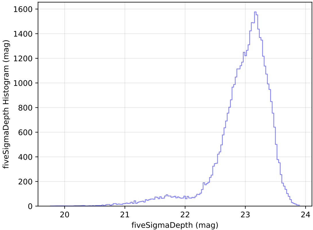
ddf_loaded_fl1_v3.4_10yrs Yr 1 z band: fiveSigmaDepth Histogram
