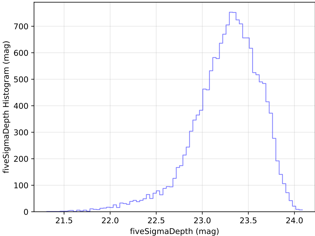
ddf_loaded_fl1_v3.4_10yrs Yr 1 u band: fiveSigmaDepth Histogram
