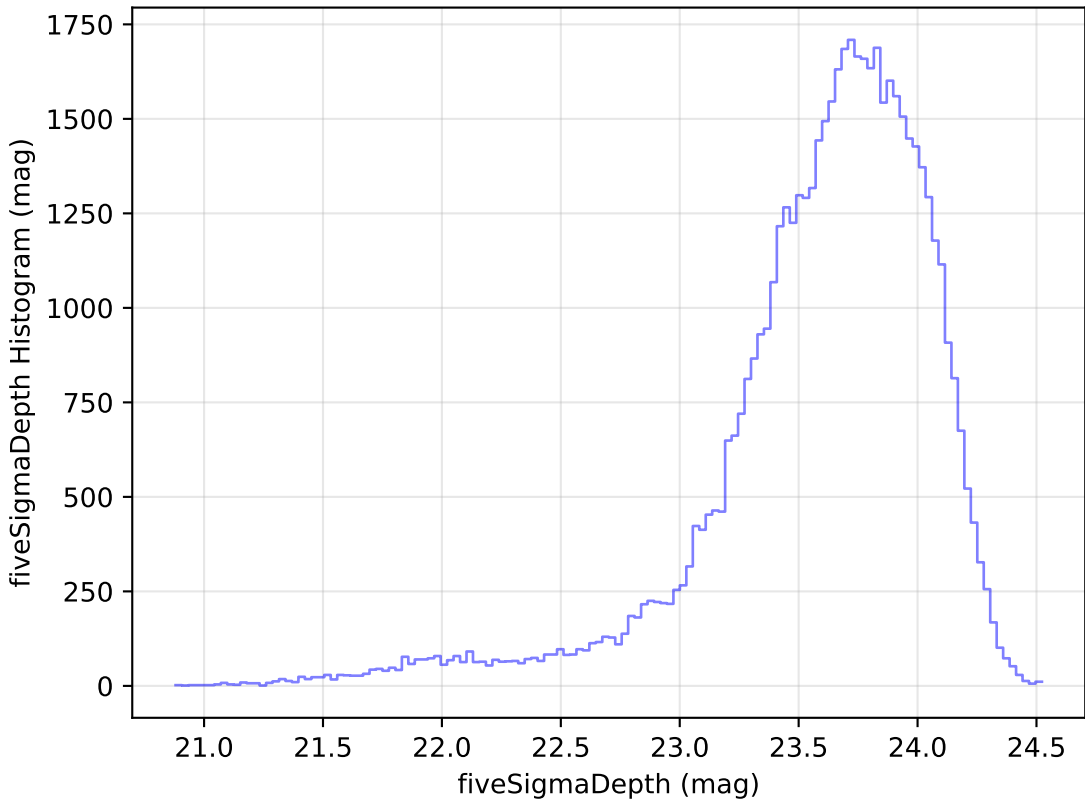
ddf_loaded_fl1_v3.4_10yrs Yr 1 i band: fiveSigmaDepth Histogram
