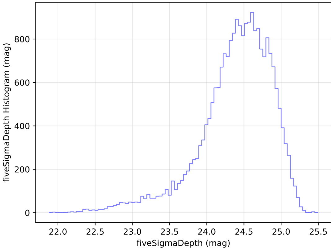
ddf_loaded_fl1_v3.4_10yrs Yr 1 g band: fiveSigmaDepth Histogram
