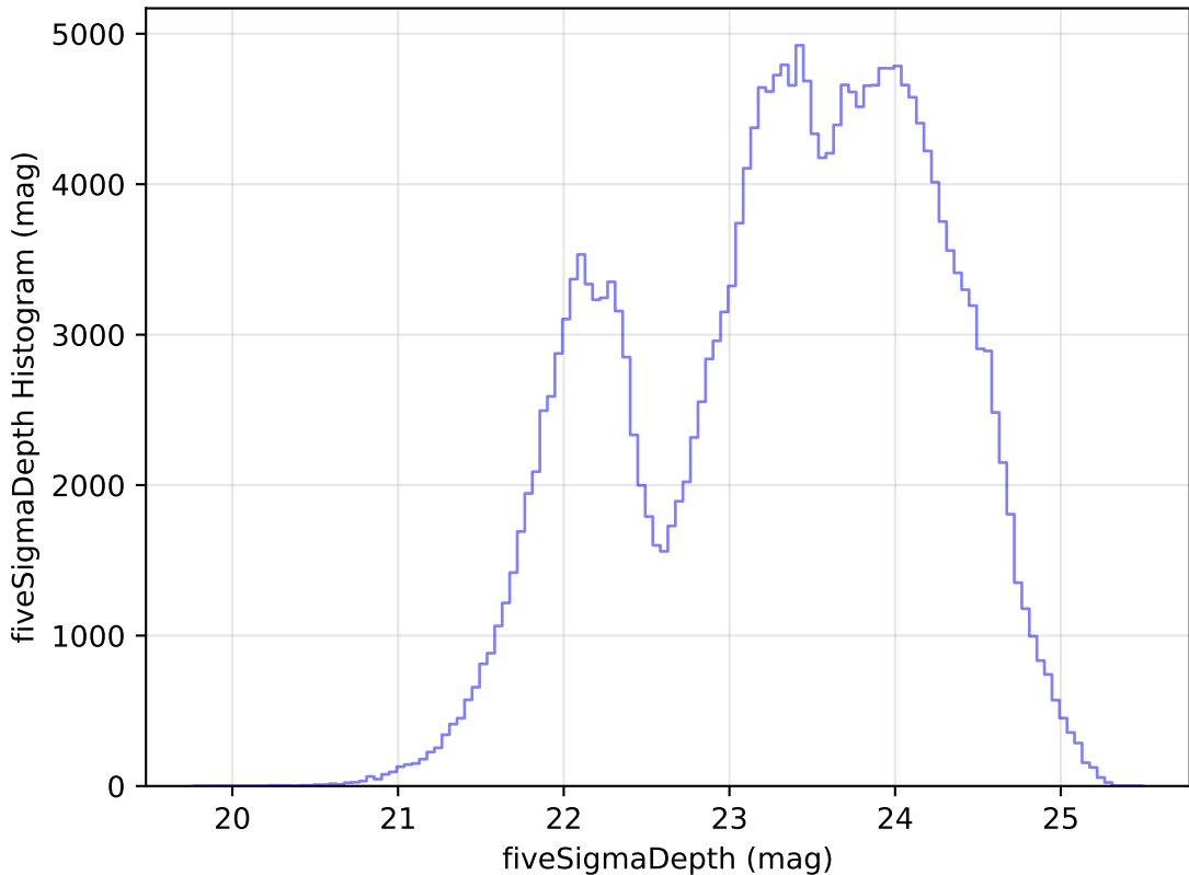
ddf_loaded_fl1_v3.4_10yrs Yr 1 all bands: fiveSigmaDepth Histogram
