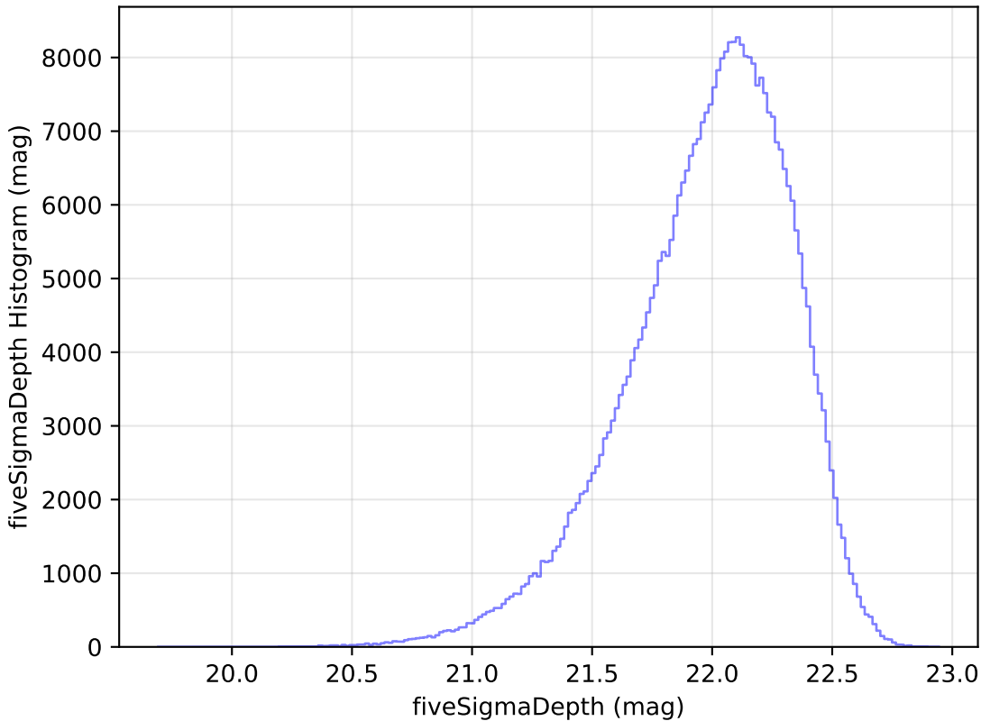
ddf_loaded_fl1_v3.4_10yrs WFD y band: fiveSigmaDepth Histogram
