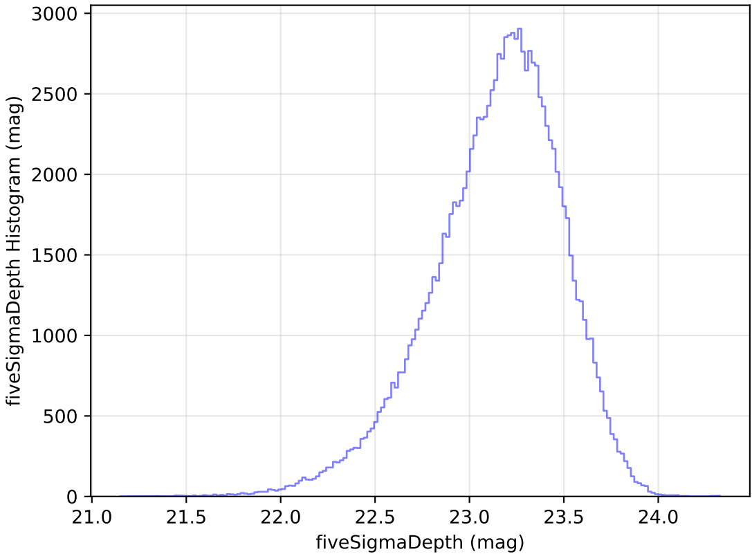
ddf_loaded_fl1_v3.4_10yrs WFD u band: fiveSigmaDepth Histogram
