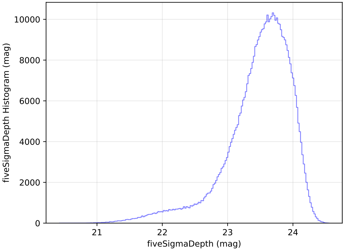
ddf_loaded_fl1_v3.4_10yrs WFD i band: fiveSigmaDepth Histogram
