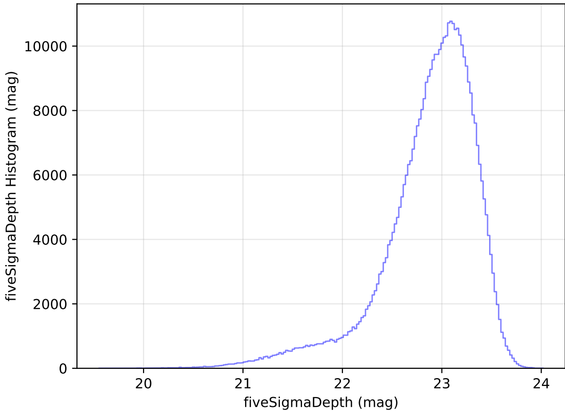
ddf_loaded_fl1_v3.4_10yrs All sky z band: fiveSigmaDepth Histogram
