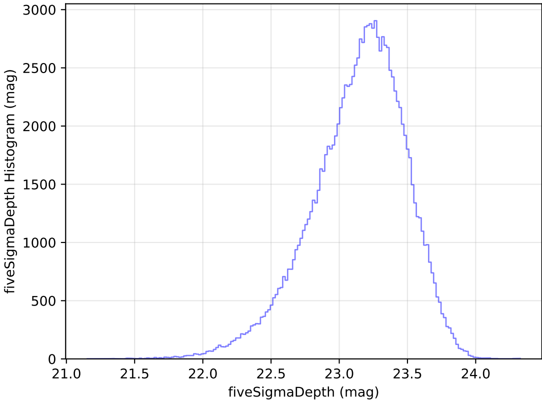
ddf_loaded_fl1_v3.4_10yrs All sky u band: fiveSigmaDepth Histogram
