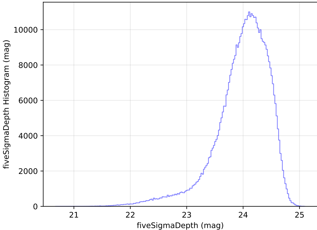
ddf_loaded_fl1_v3.4_10yrs All sky r band: fiveSigmaDepth Histogram
