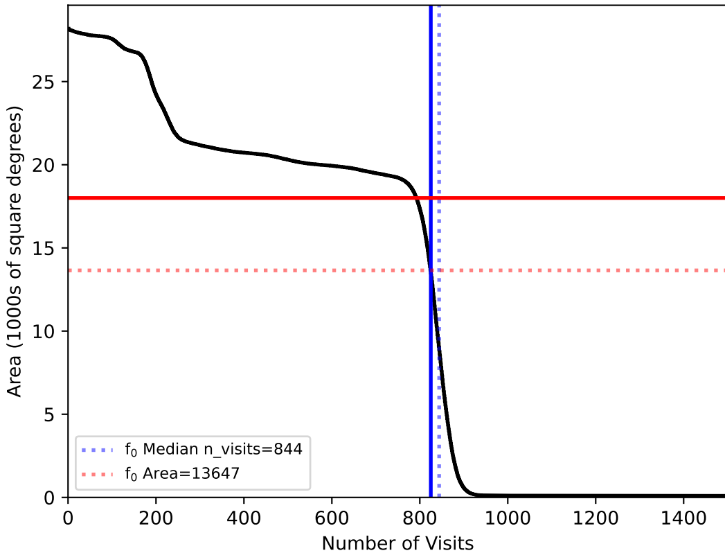
ddf_loaded_fl1_v3.4_10yrs All sky: fO
