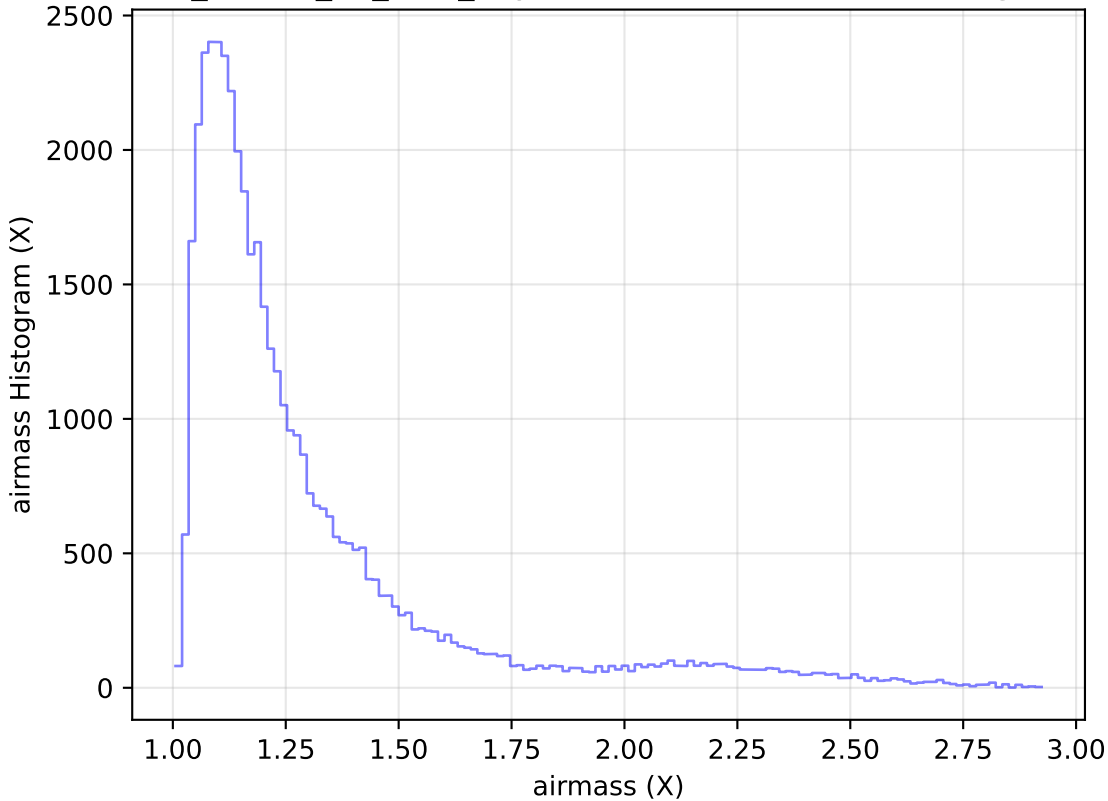
ddf_loaded_fl1_v3.4_10yrs Yr 1 z band: airmass Histogram
