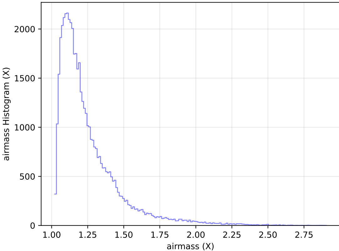
ddf_loaded_fl1_v3.4_10yrs Yr 1 y band: airmass Histogram
