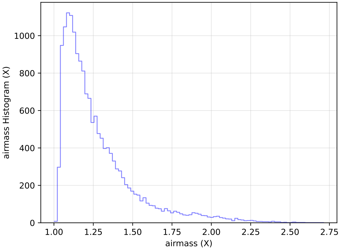
ddf_loaded_fl1_v3.4_10yrs Yr 1 u band: airmass Histogram
