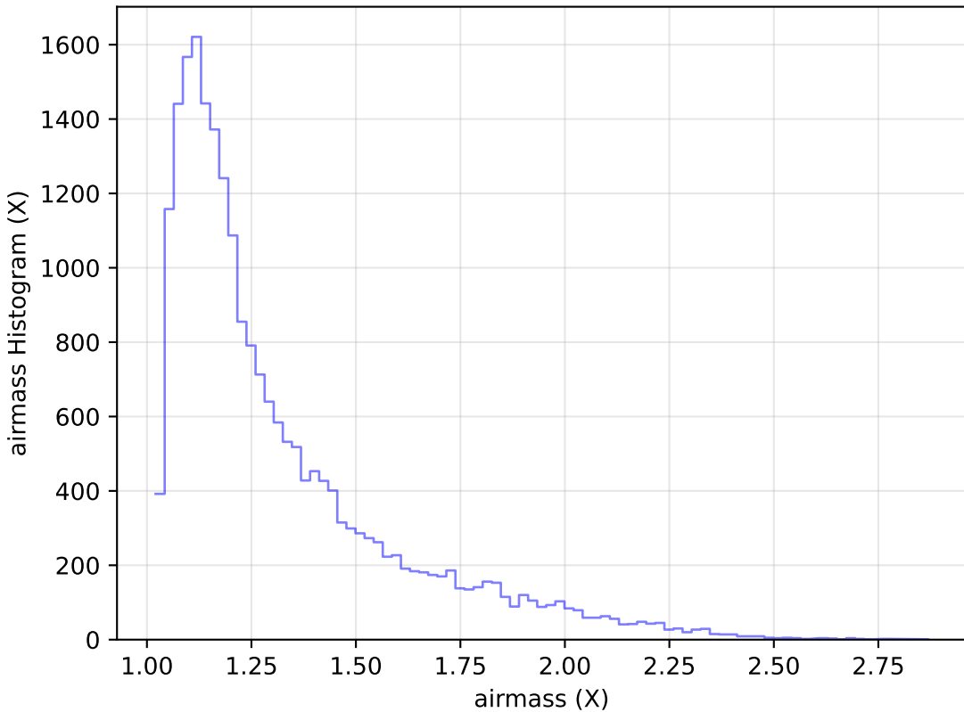
ddf_loaded_fl1_v3.4_10yrs Yr 1 g band: airmass Histogram
