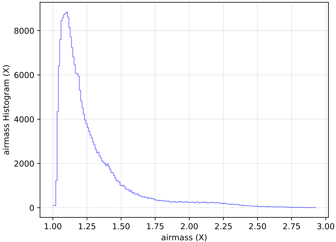
ddf_loaded_fl1_v3.4_10yrs Yr 1 all bands: airmass Histogram
