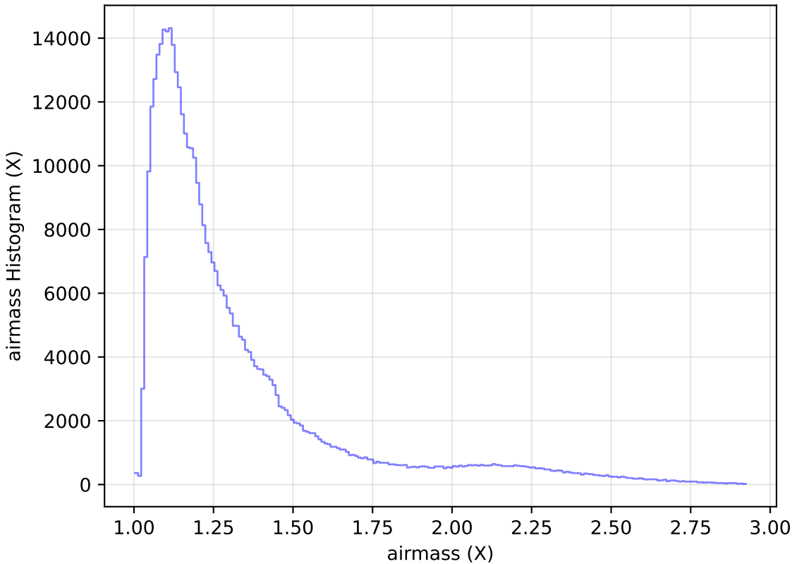
ddf_loaded_fl1_v3.4_10yrs WFD z band: airmass Histogram
