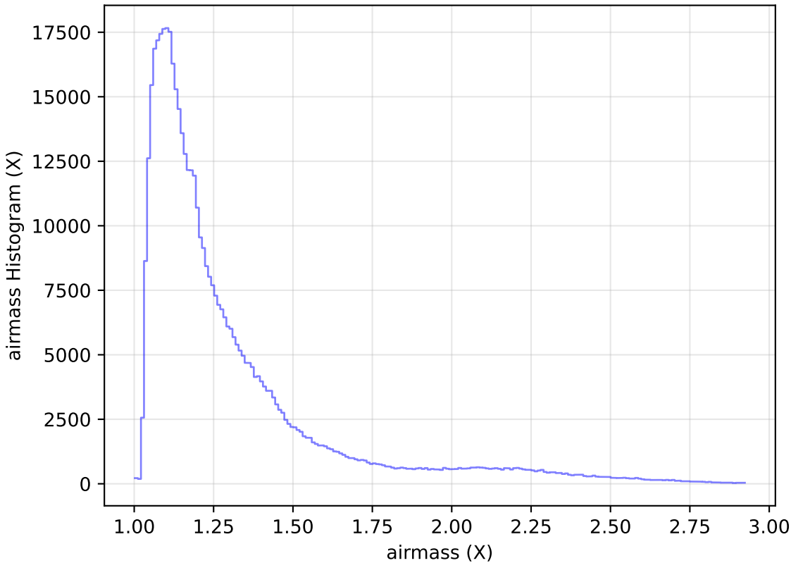
ddf_loaded_fl1_v3.4_10yrs WFD i band: airmass Histogram
